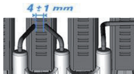
Electrodes position
